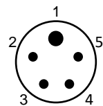
Looking at the male pins on the back of the camera
