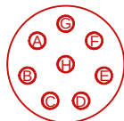
97-3108B-18-8P BACKVIEW
