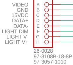
97-3108B-18-8P BACKVIEW
